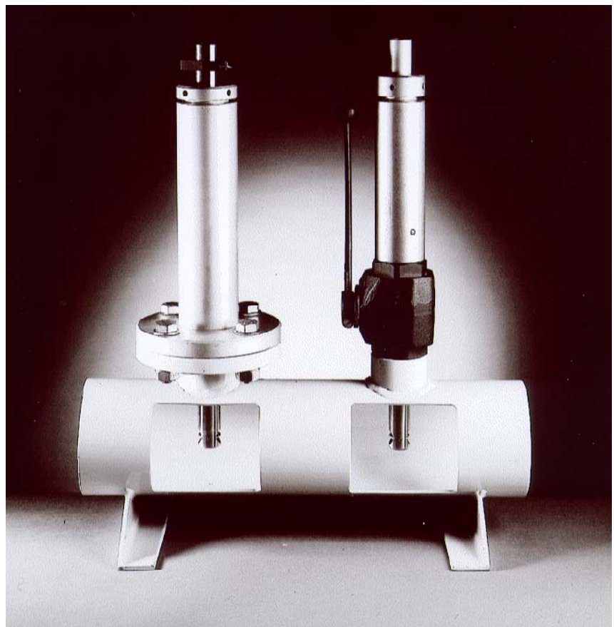
Probe guide piece with clamp
